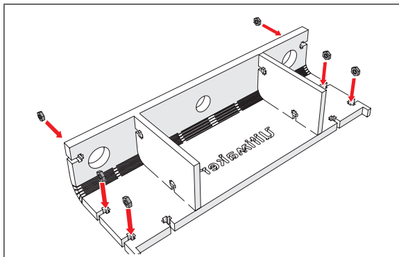
image 81: Placing the Hex nuts in the T-slots
