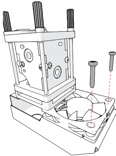
image 62: attaching the fan to the metal fan duct.
