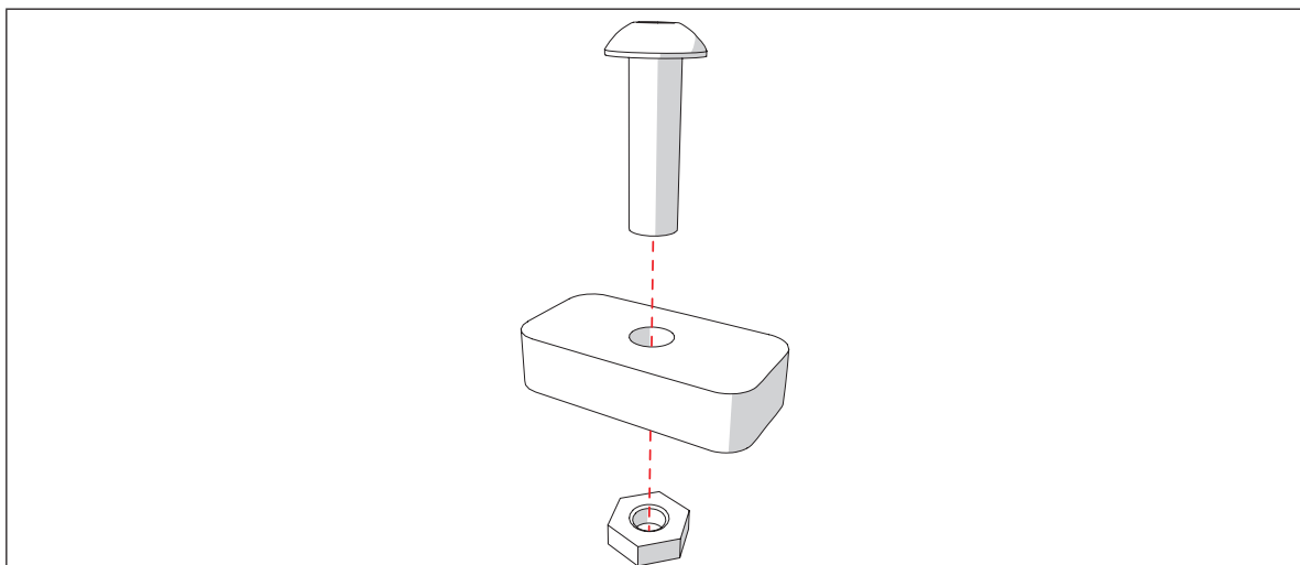
image 30: assembling wooden parts, marked C
