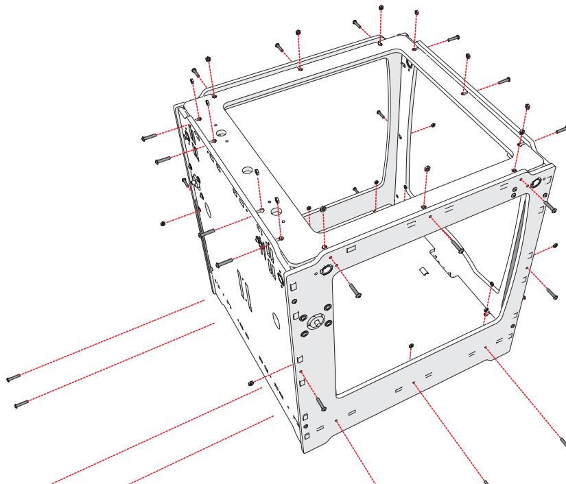
image 19: complete the frame by checking if all the bolts are tightened
