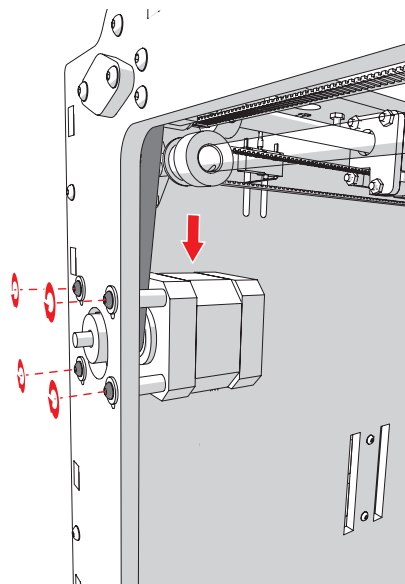
image 70: tightening the bolts of the Y motor.
