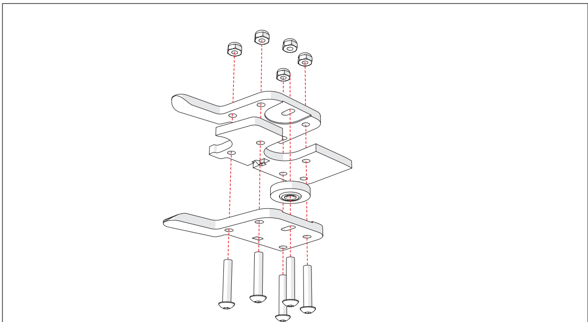
image 96: placing the side plates over the mounting plate
