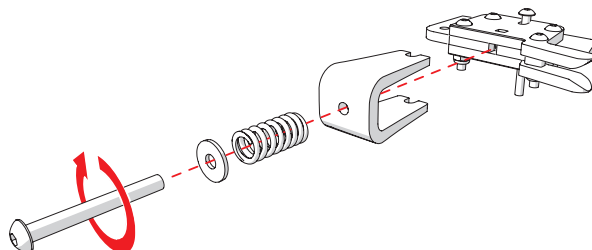
image 97: placing the U-Bracket on the clamp assembly
