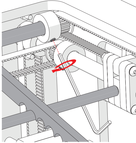
image 69: adjusting the timing pulleys
