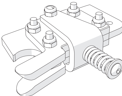
image 98: result after attaching the U-Bracket on the clamp assembly
