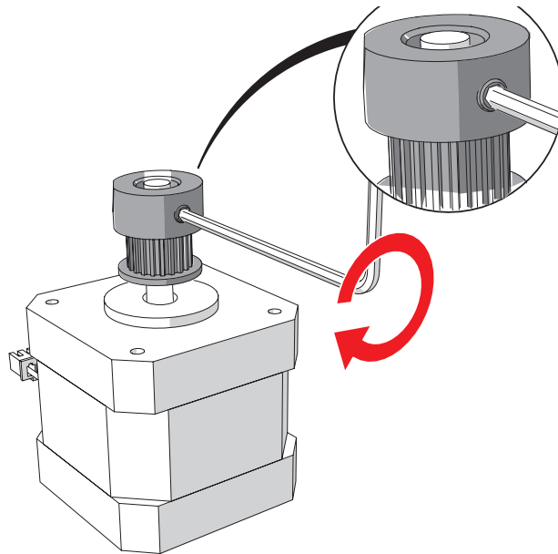
image 9: placing the pulley on the Y motor axis
