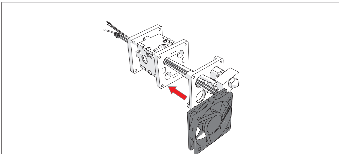
image 57: moving the wires of the thermocouple, cartridge heater and the small fan through the wooden part TOP
