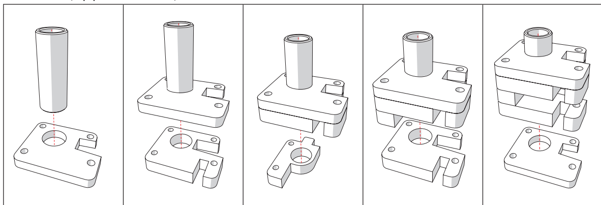
image 25: assembling the LEFT slider block
