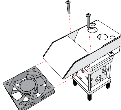
image 61: attaching the back of the fancap and fan.
