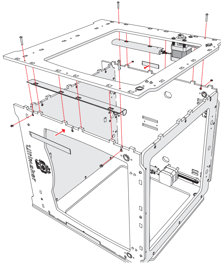
image 18: positioning the other SHORT and LONG cable ducts and attaching the LEFT panel
