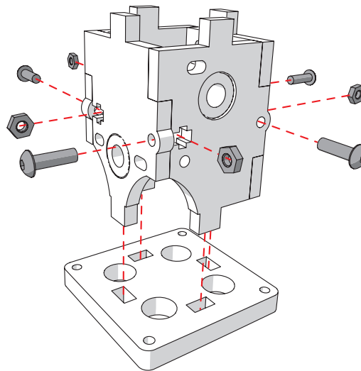
image 51: attaching the sides together and placing into wooden part 8B.
