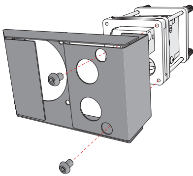
image 60: attaching the front of the fancap
